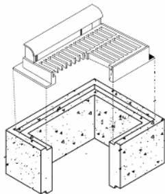
Lift grate and seat StormBasin on frame
