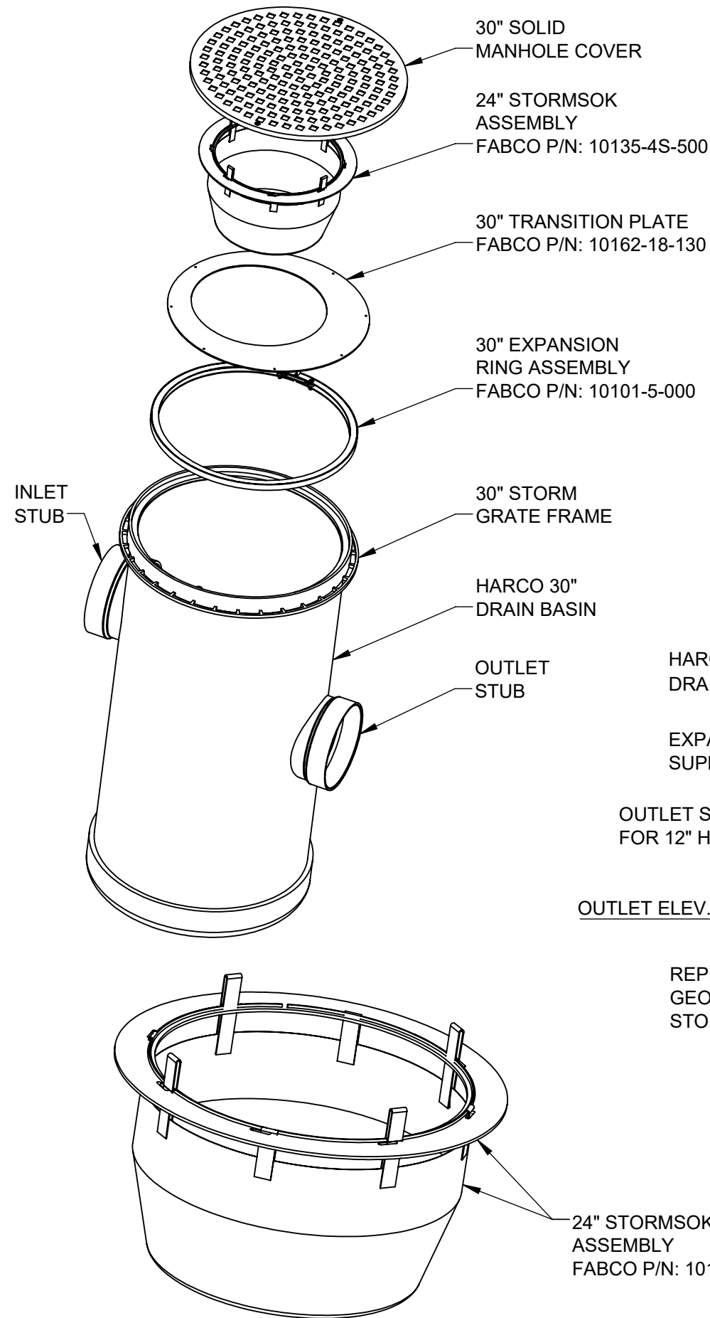
REFERENCE VIEW
