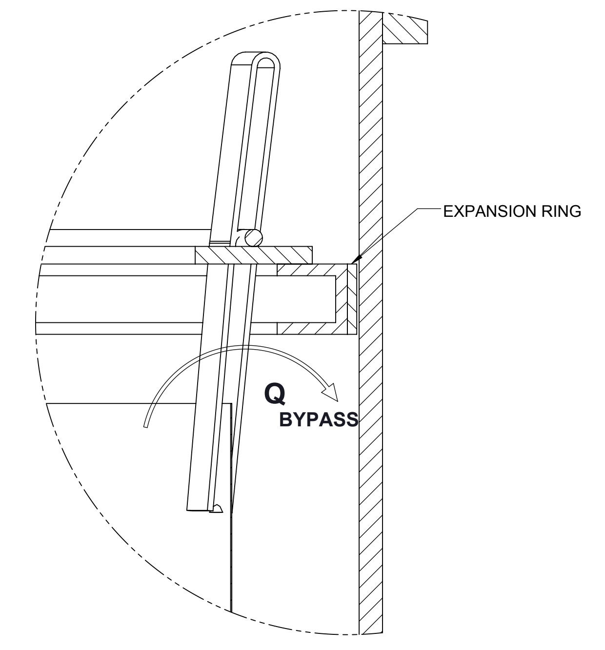
DETAIL 1
