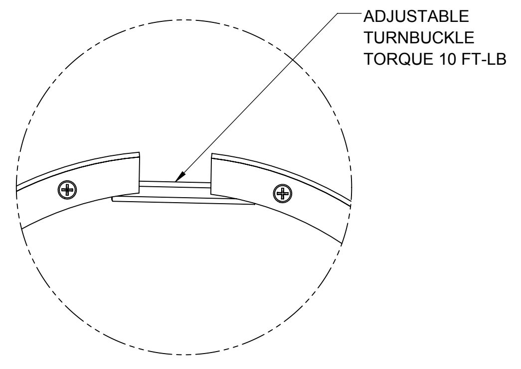
CUTAWAY DETAIL
