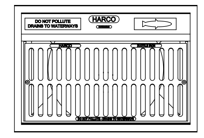
STORMSOK FITS 2 X 2 HARCO 15" CURB INLET
