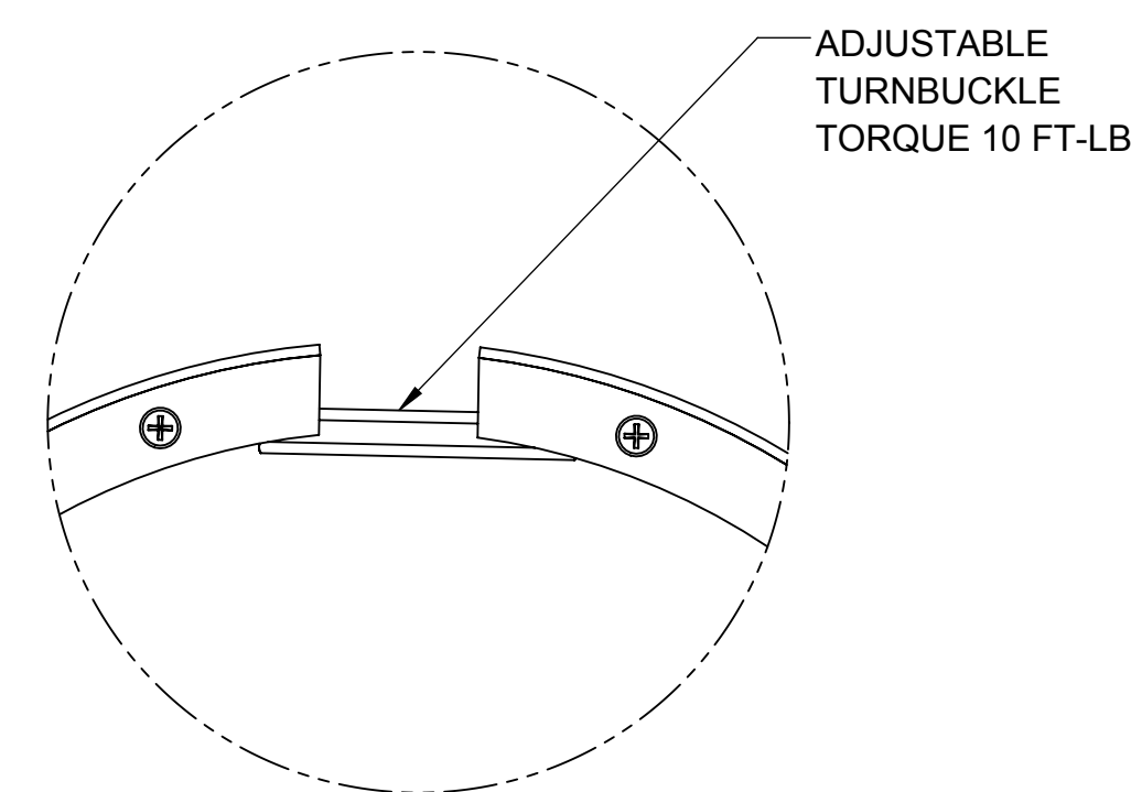
CUTAWAY DETAIL
