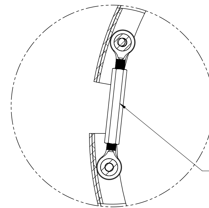
CUTAWAY DETAIL
