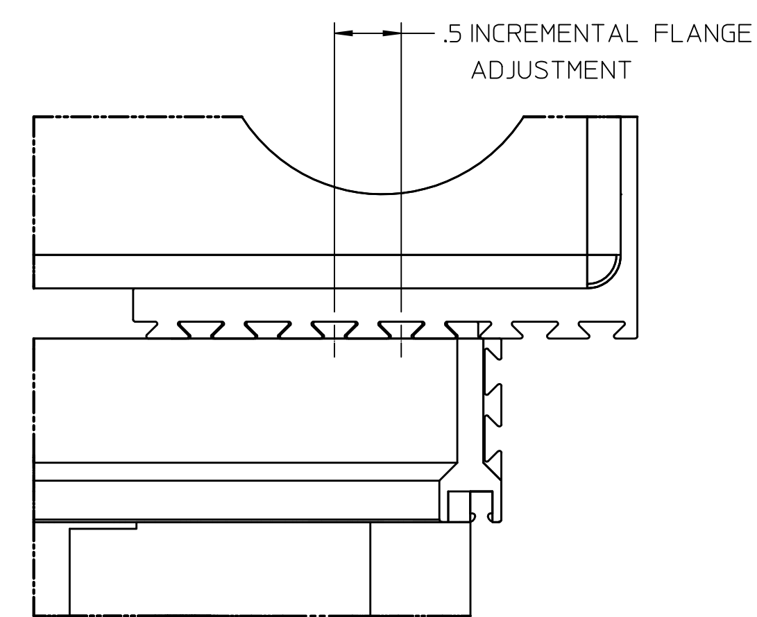
DETAIL 1 SCALE 1:1
